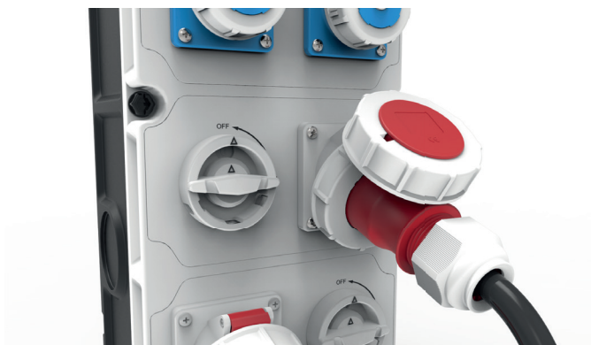
Detailed view of switched interlocked flange plate.
